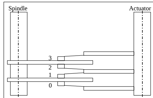
MPD3129AT Model
