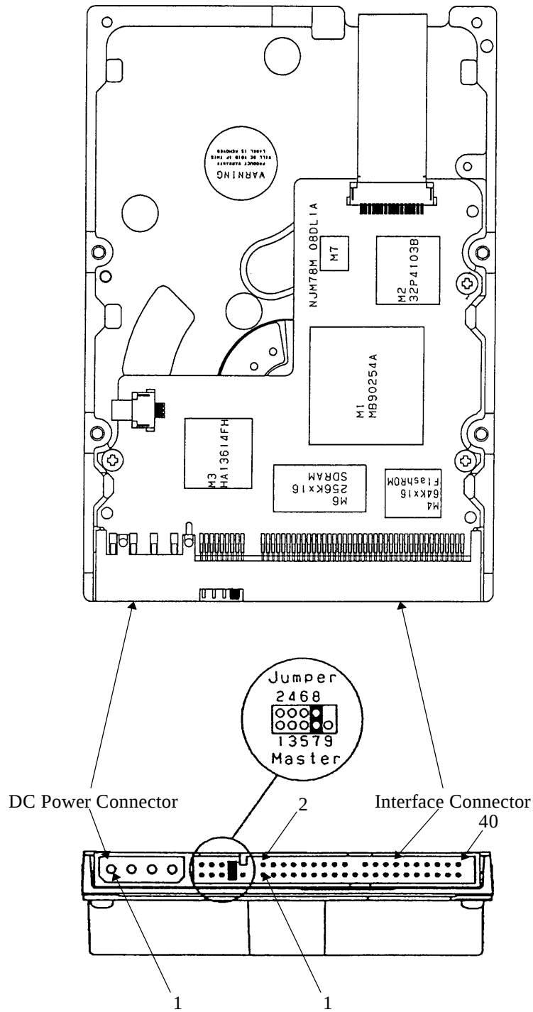
Figure 3.10 Jumper location
