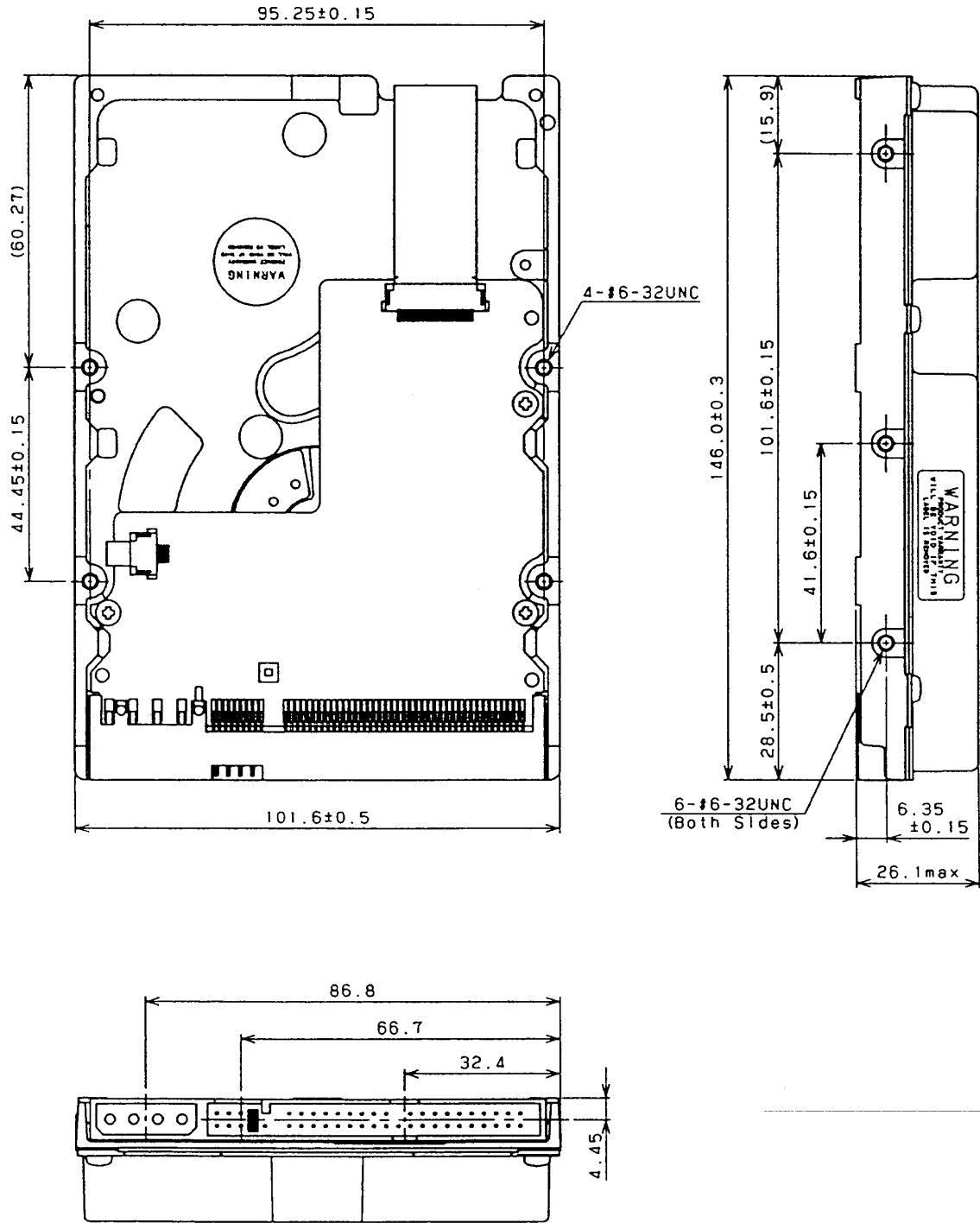
Figure 3.1 Dimensions
