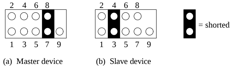
Figure 3.12 Jumper setting of master or slave device
